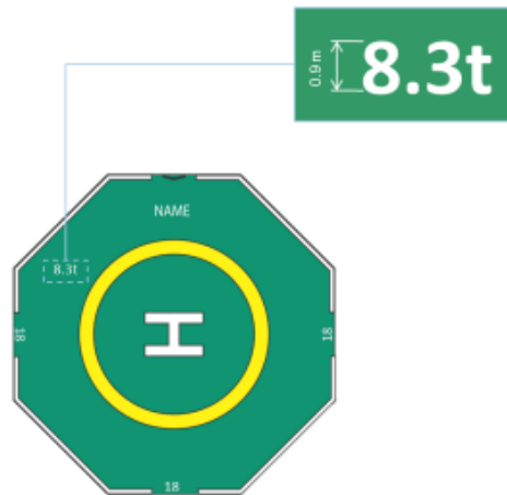
Appendix Figure 13.12 Maximum Allowable Mass Marking (Typical) - Offshore
