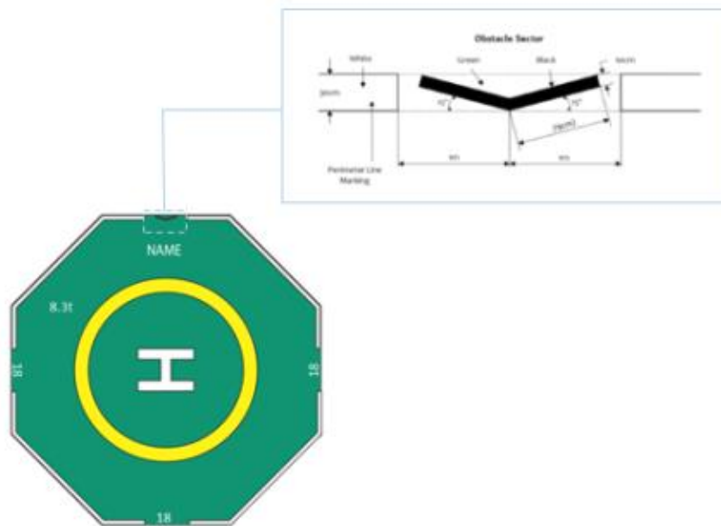
Appendix Figure 13.16 Helideck Chevron - Offshore
